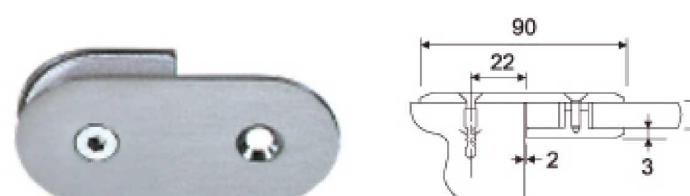
M-507 180° Single Semi-circle
