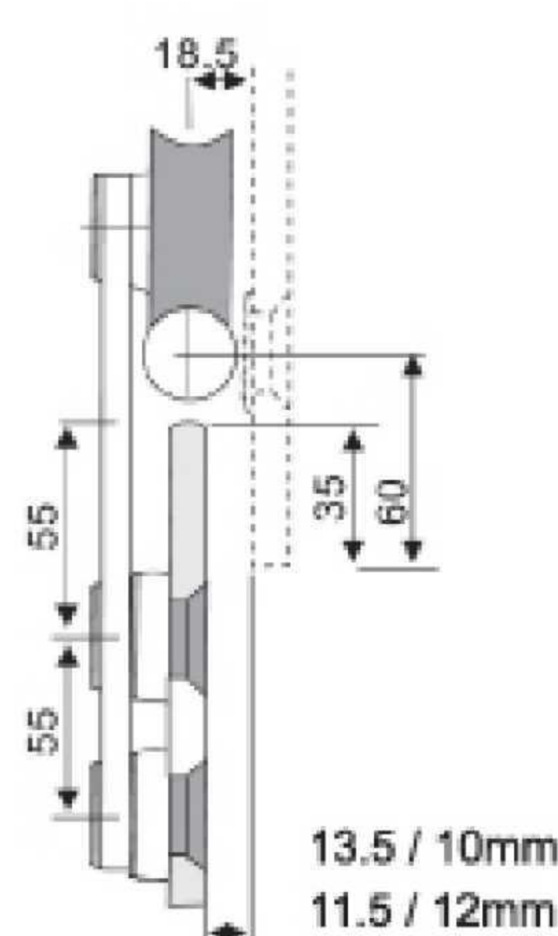
Φ25圆管截面安装图 Φ25 Sectional installation indication of elliptical pipe
