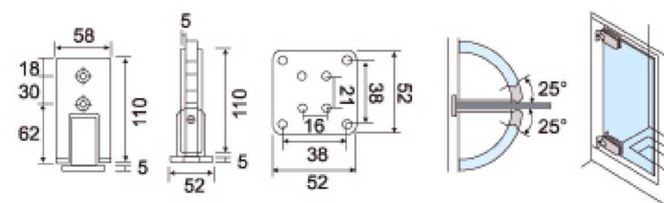
M-324 Rectangle 90° Double
