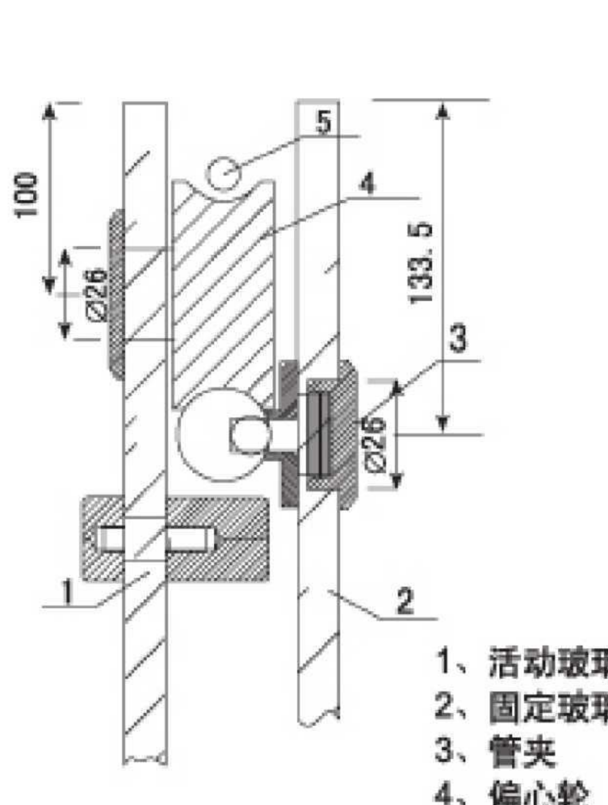
Φ25管浴室吊轮截面安装图 Sectional installation of Φ25 pipe bathroom hanging wheel
