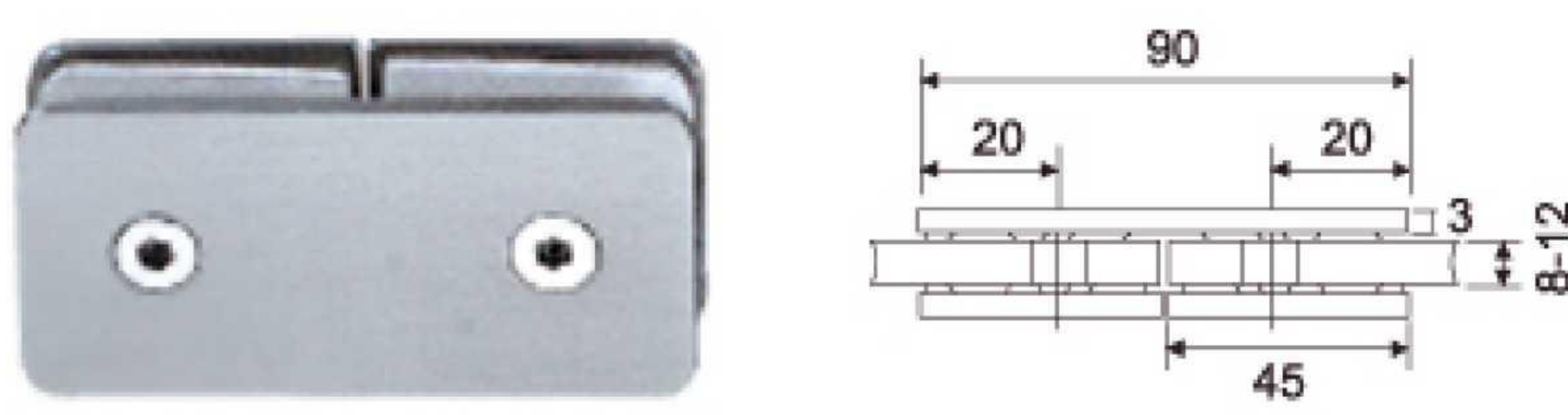
M-518 180° Double Straight
