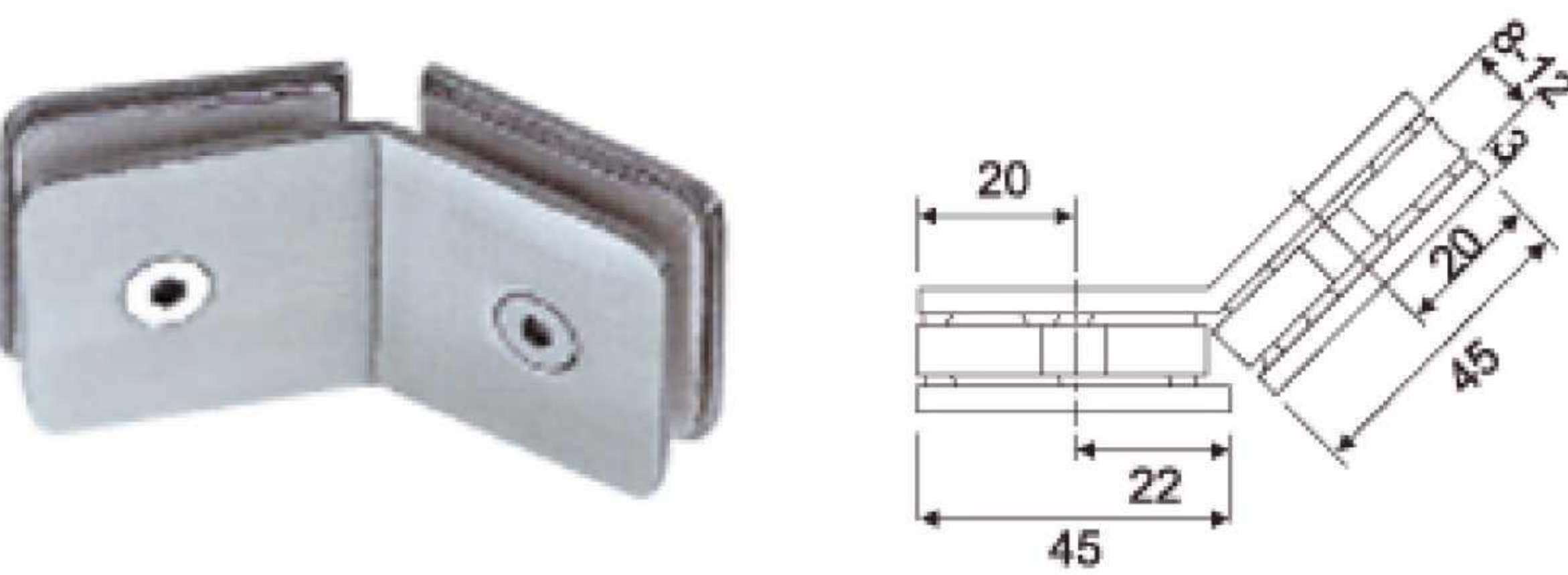
M-516 135° Double Straight
