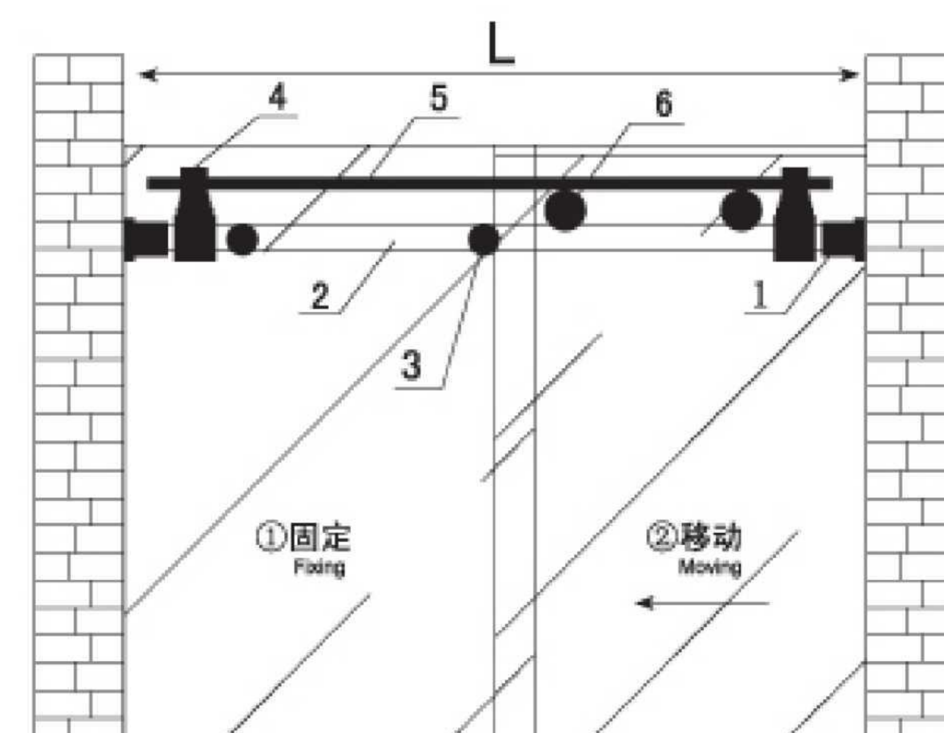
Φ22管浴室吊轮平面安装图 Installation of Φ22 pipe bathroom hanging wheel
