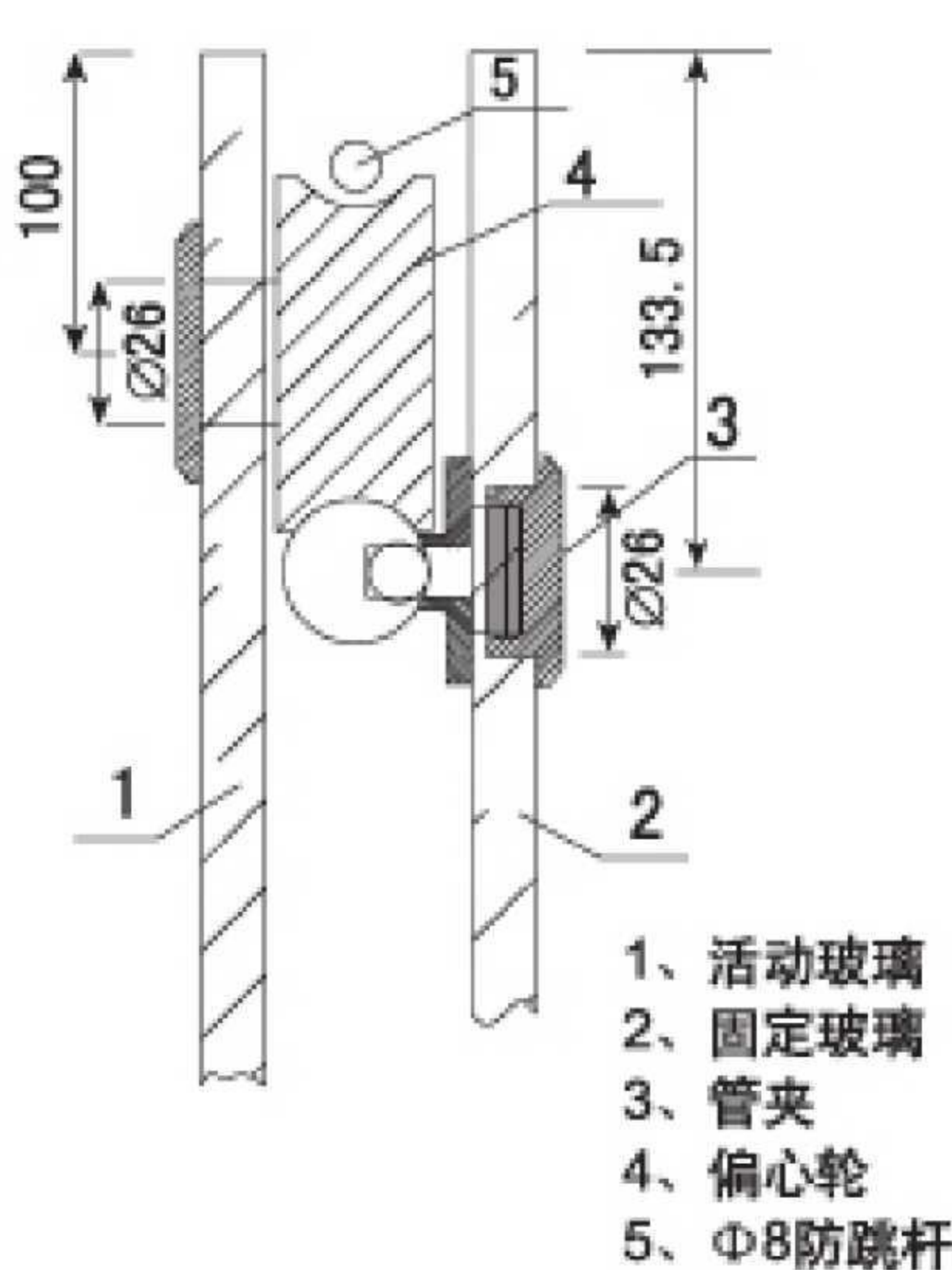
Φ22管浴室吊轮截面安装图 Sectional installation of Φ22 pipe bathroom hanging wheel
