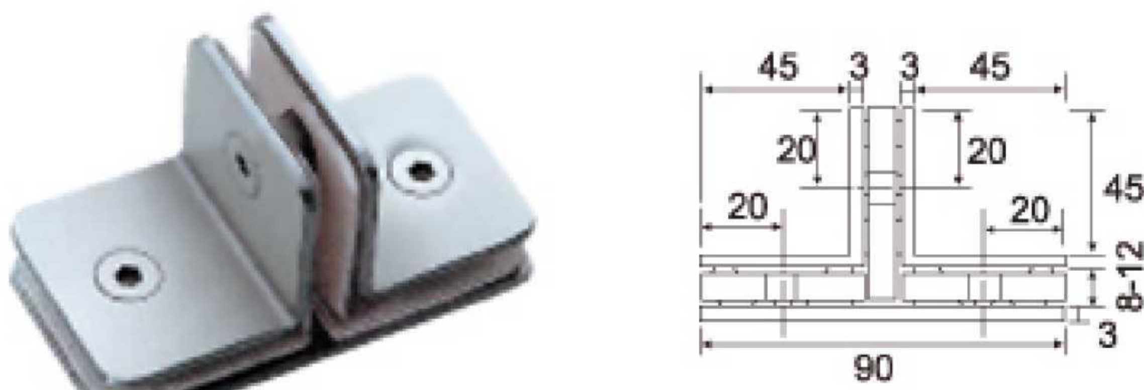
M-519 Party T Shape
