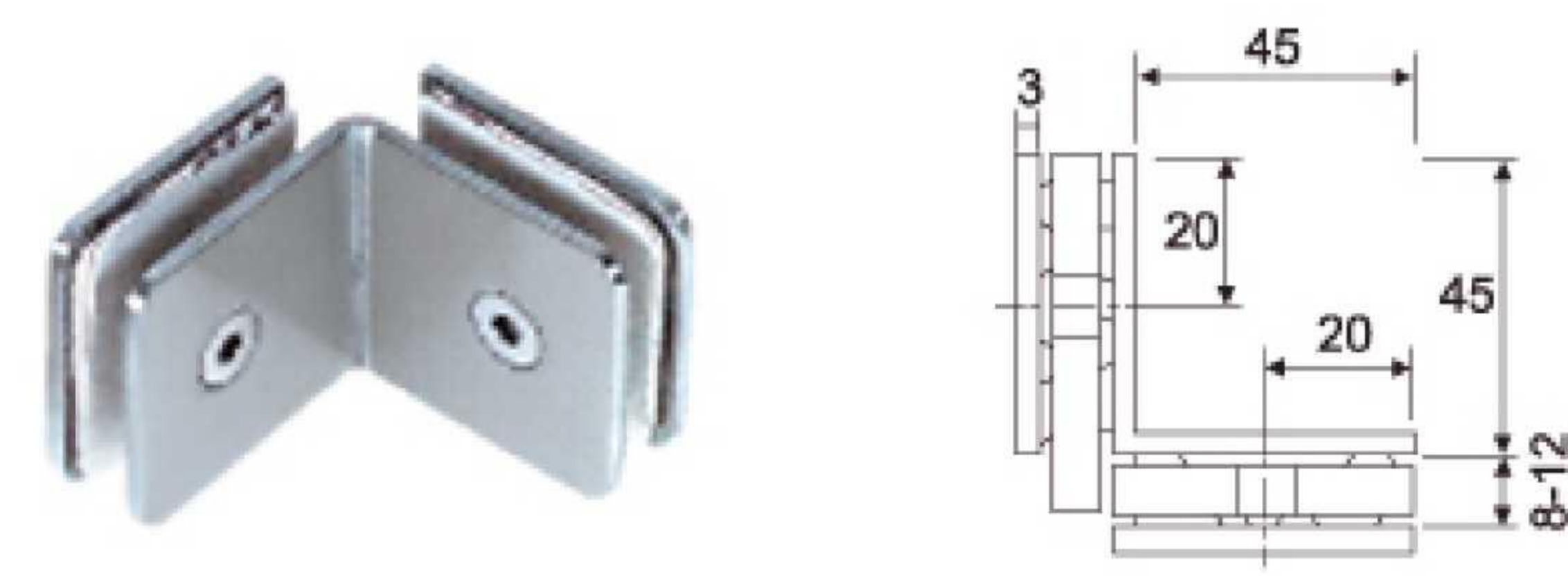
M-514 90° Double Straight
