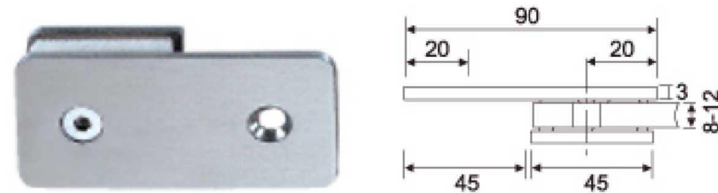
M-517 180° Single Straight
