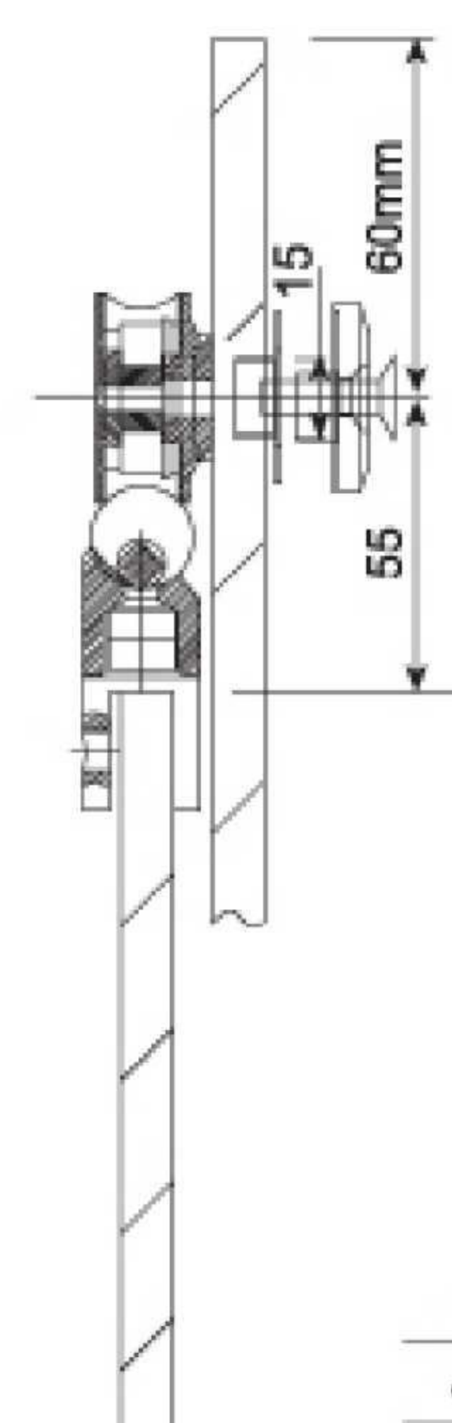
截面安装图 Sectional installation indication
