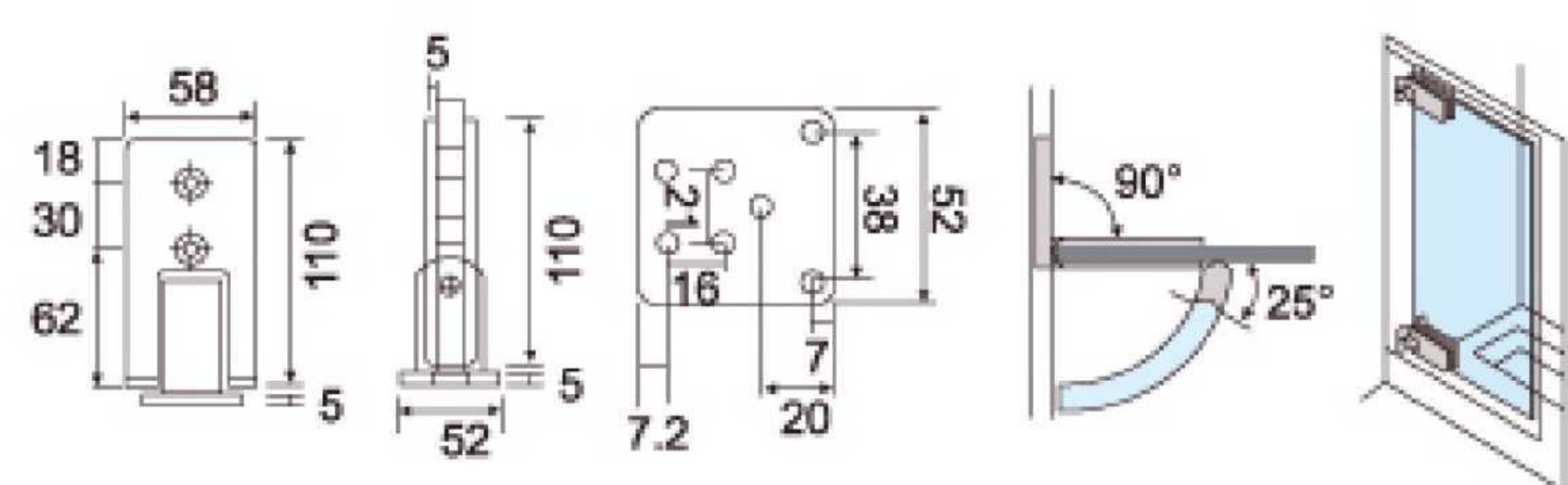
M-323 Rectangle 90° Single
