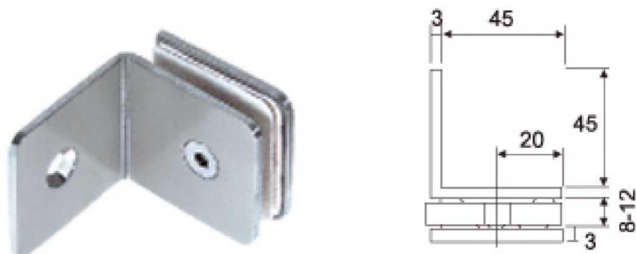
M-513 90° Single Straight
