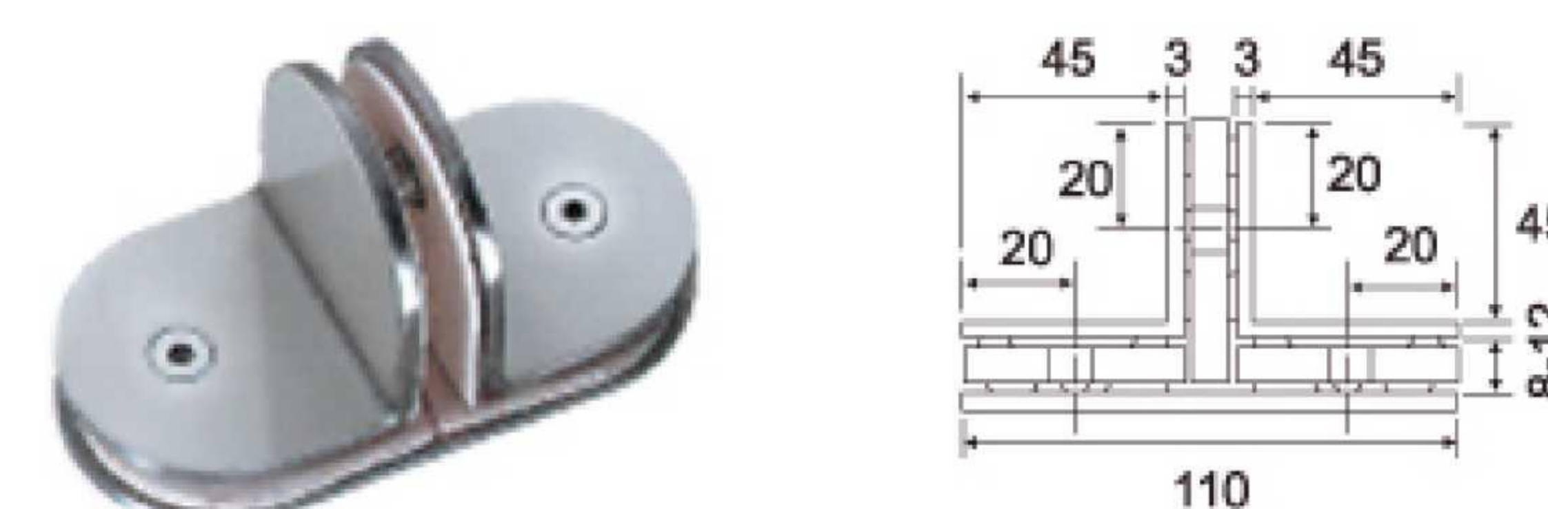
M-509 Semi-circle T Shape
